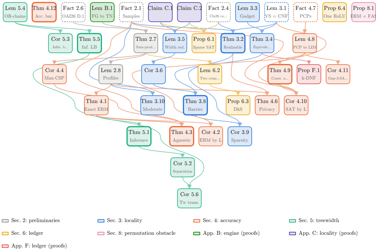
Figure 2: Dependencies between the results. An arrow from X to Y means that the proof of Y cites X , after transitive reduction. Dashed frames mark imported theorems, thick frames mark the main theorems, and hypotheses are not drawn. Theorem 4.12 and Propositions 8.1 and 6.4 use no other result of this paper.
